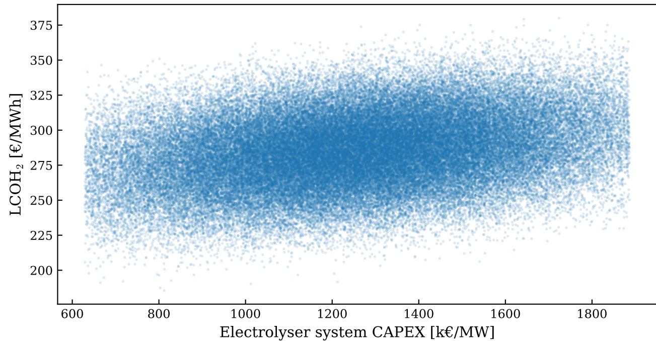
LCOH 2 vs Electrolyser CAPEX
